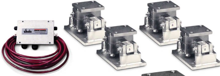
Fabricated stainless steel module with RL75016SS double-ended beam load cell.
